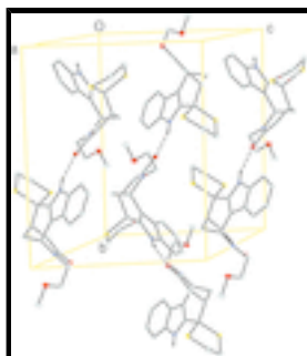
Fig. 2. A partial packing diagram of the title compound. Hydrogen bonds are shown as dashed lines. H atoms not involved in hydrogen bonding have been omitted for clarity.
